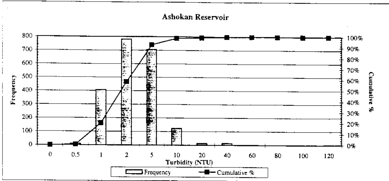
Figure 1A Catskill Reservoir System Turbidity Probability Distribution - 1987 to 1994
