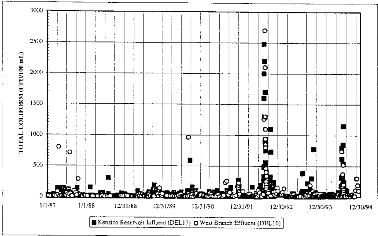
Figure 3C Delaware Aqueduct Impact of West Branch Reservoir on Total and Fecal Coliform DEL10/DEL17 Comparison
