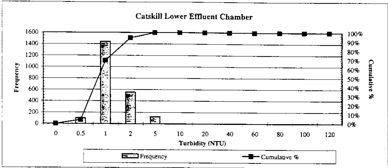
Figure 1B Comparison between Catskill Lower Effluent Chamber and Shaft 18 (DEL18) Turbidity Probability Distribution - 1987 to 1994
